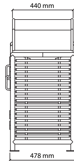
Side View
